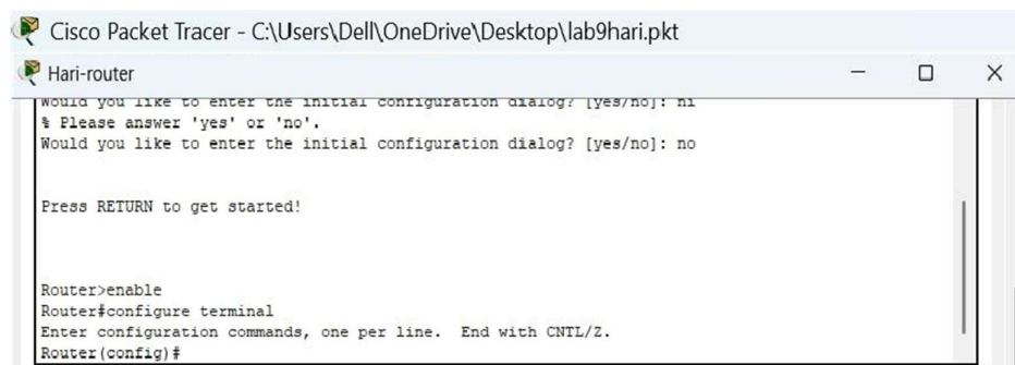
Fig: Entering Privileged EXEC and Global Configuration Mode on the Router
