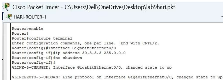
Fig: Configuring IP Address on Gigabit Ethernet Interface
