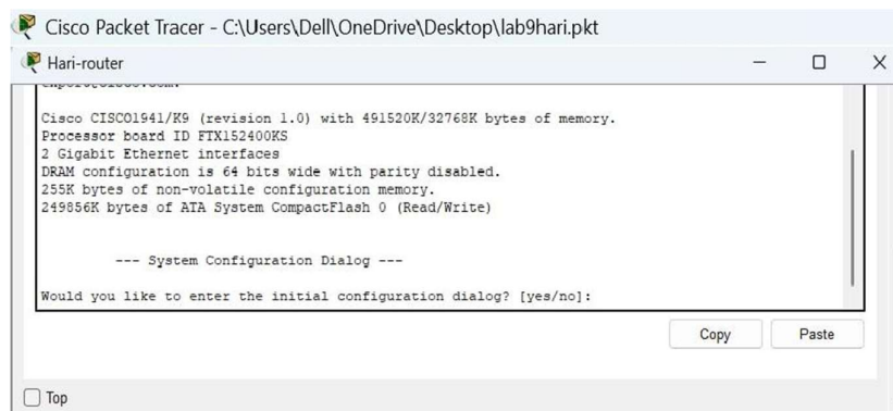
Fig: Accessing Router Command-Line Interface via Console Cable
