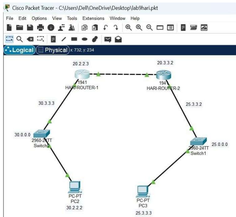
Fig: Network Diagram for static routing
